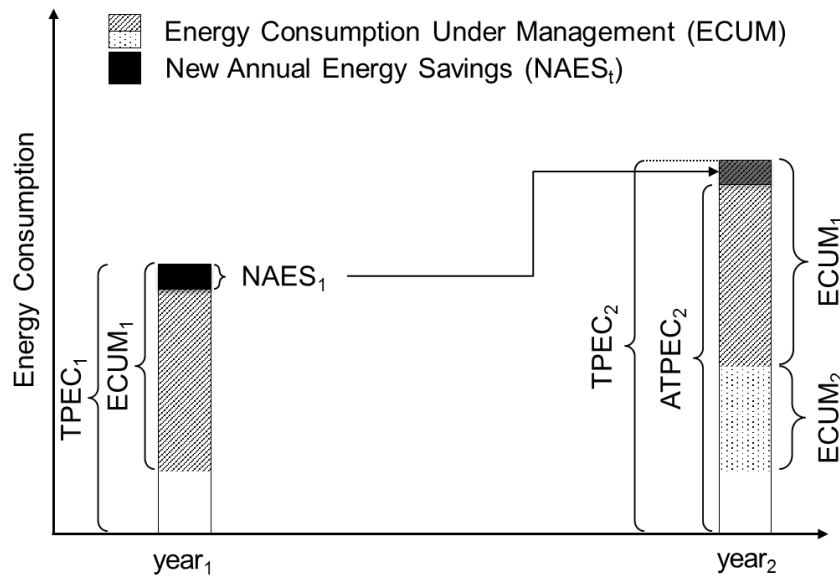
Figure 14: Total Projected Energy Consumption and Adjusted Total Projected Energy Consumption
