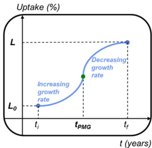
Figure 9: Standard logistic function
