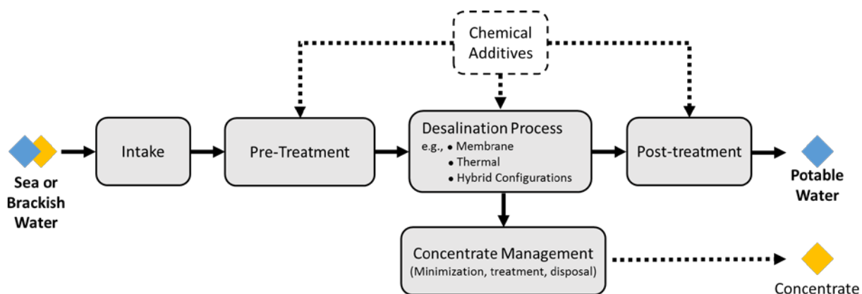
Figure 2-2. Simplified Five-Unit Operation Desalination System Process Flow Diagram
