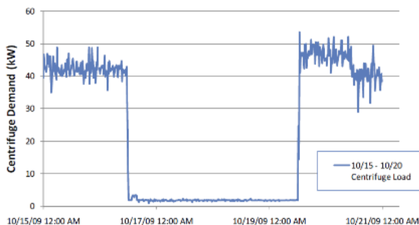
Figure 17: Centrifuge demand reduction from shutting down both centrifuges.
