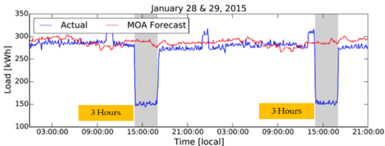
Figure 19: Three hour DR events at WPCP with day-ahead notification
